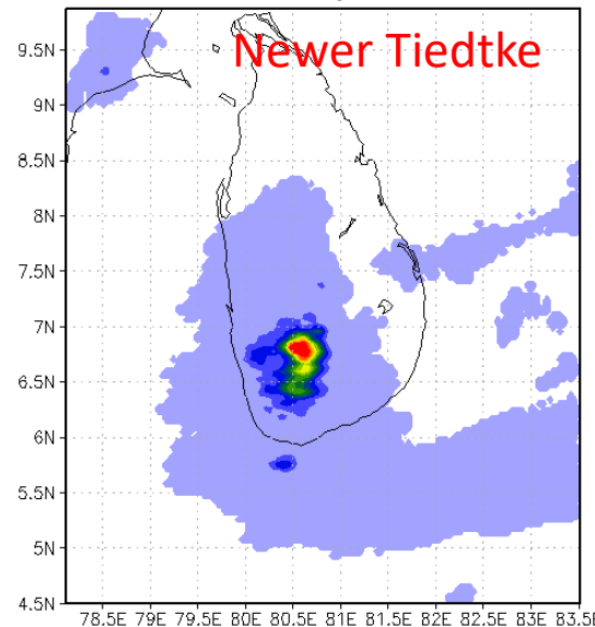
Rainfall 25May2017 16,0
