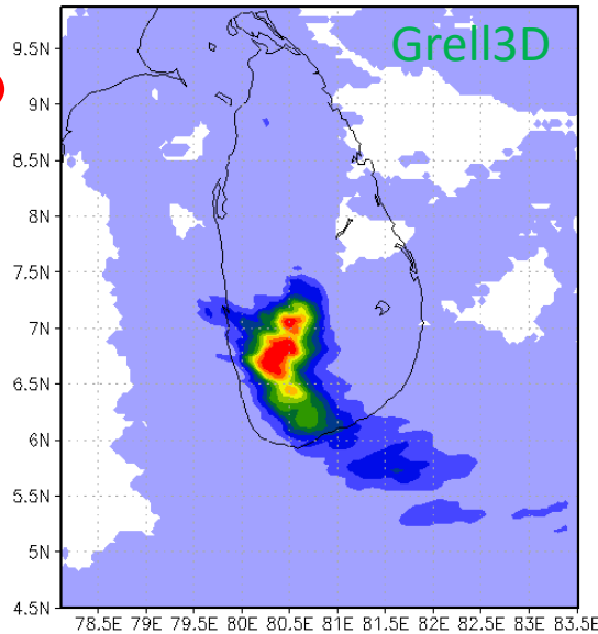
Rainfall 25May2017 5,0
